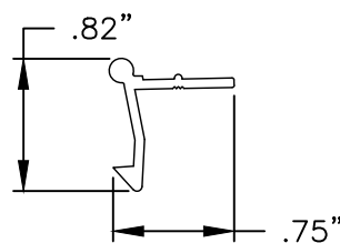
PINCH LOCK 6063-T5
